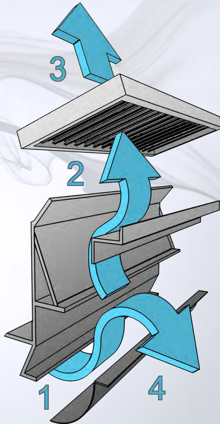
Inside the Wetrex™; baffles, impellers & filters
